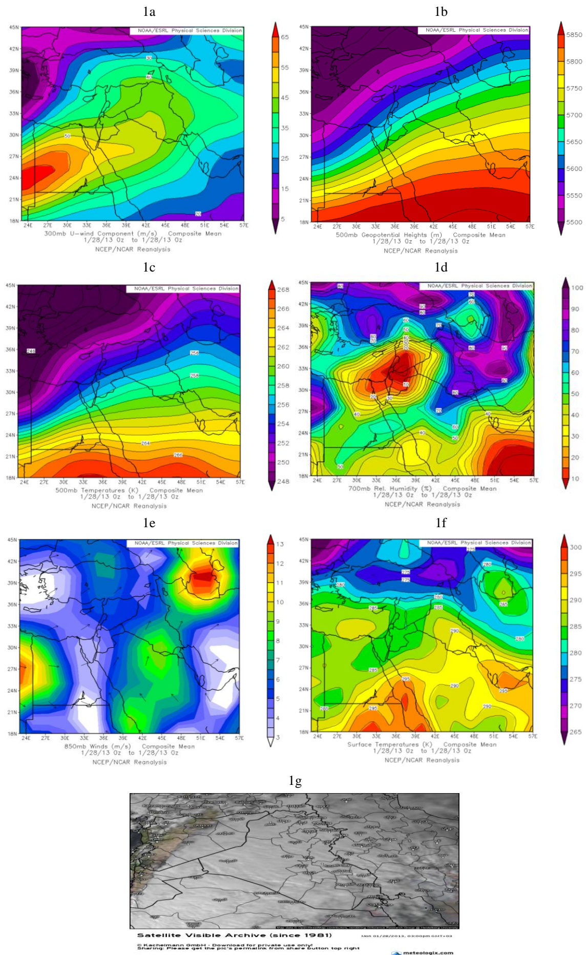
Figure 1. All level chart sand satellite image of the case (28/01/2013).
