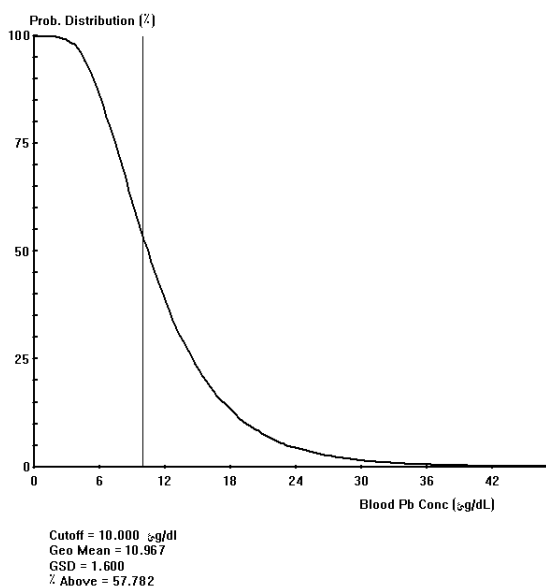
Figure 3. Dispersion curve for the mean parameter with Geometric means of 10.96.
