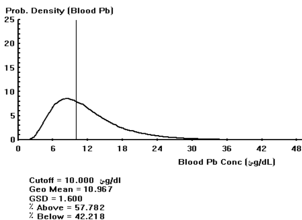
Figure 2. The density of blood Pb levels BLL spoke to anticipated qualities at cut-off degrees of <10 \mu\text{g/dL} .
