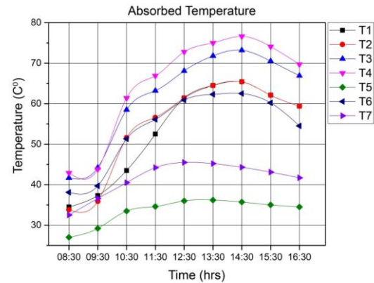
Figure 2. The temperature change of the parts of the solar distillation with the temperature of ambient air.
