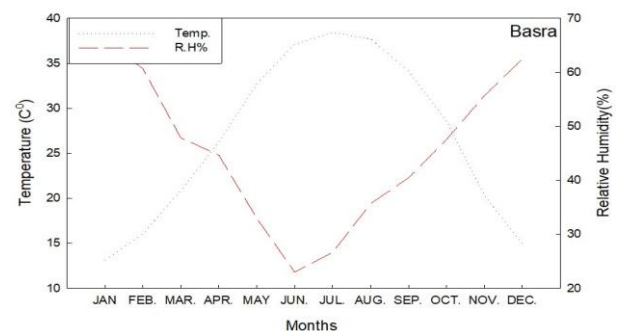
Figure 3. The Monthly Average of Temperature and Relative Humidity for Basra station (2000-2014).
