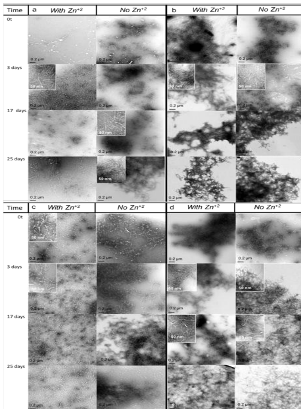
Figure 1: Electron microscopy images of peptides 1- 4 self-assembled with/without 1mM \text{ZnCl}_2 in 25mM Tris-base buffer, pH 8. Morphology of peptides followed over 25 days.
