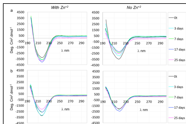
Figure 2: The CD spectra of two examples: peptide 3 and 4 assembled at 37^\circ\text{C} in the presence (left) and absence (right) of zinc over 25 days. a) peptide 3 and (b) peptide 4.
