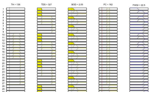
Figure 4. Matlab Rule viewer showing the inputs and the output used in FLIS
