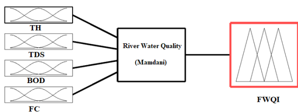
Figure 2. Membership functions of the FWQI.
